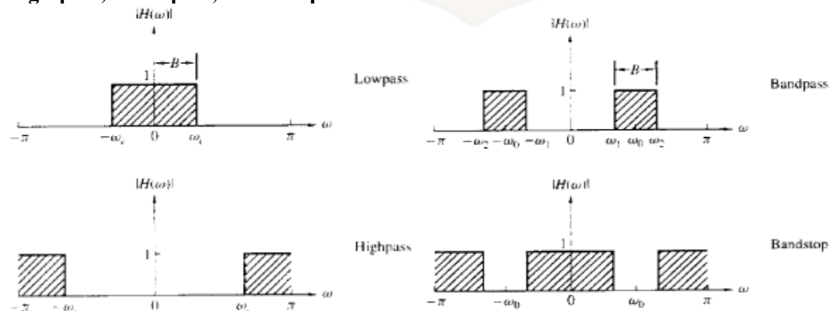
Figure: Magnitude responses for some ideal frequency-selective discrete-time filters.
